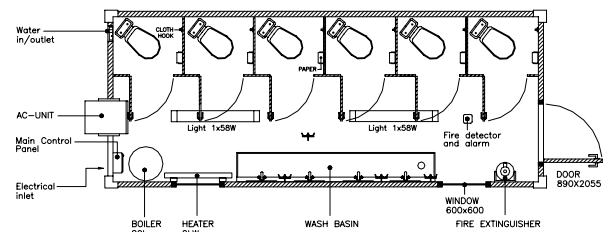
An example of a toilet container
