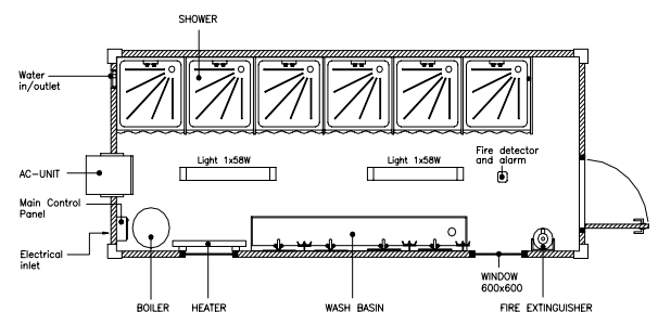
An example of a shower container
